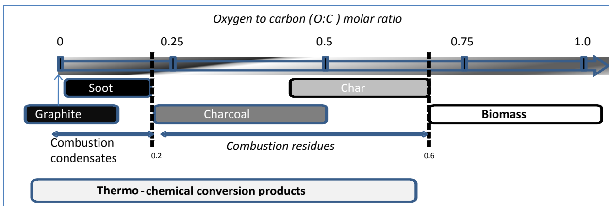
Figure 1. The spectrum of combustion product continuum as related to product O:C molar ratio. Redrawn from Spokas (2010), which was originally adapted from Hedges et al. (2000) and Elmquist et al. (2006).
